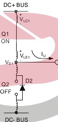
Figure 10: V_s positive
