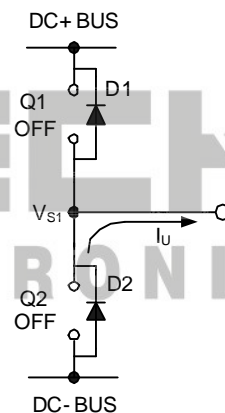
Figure 8: D2 conducting
